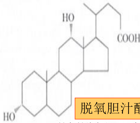
Deoxycholic acid
