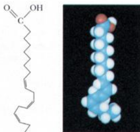
α-Linolenic acid
