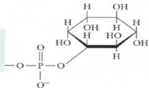
Phosphatidylinositol
