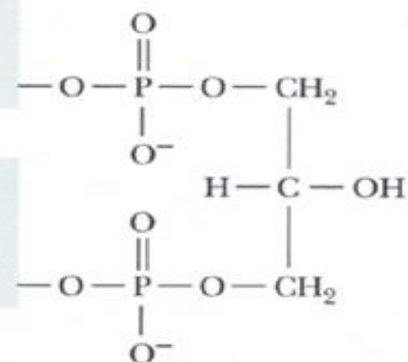
Diphosphatidylglycerol (Cardiolipin)
