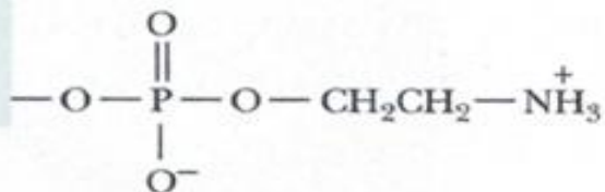
Phosphatidylethanolamine
