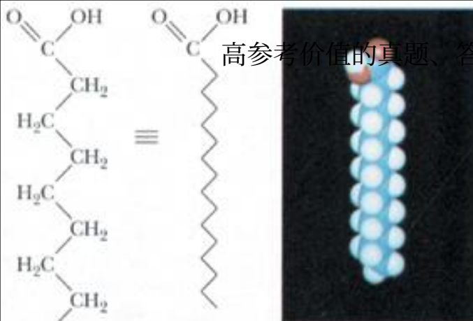
Palmitic acid
