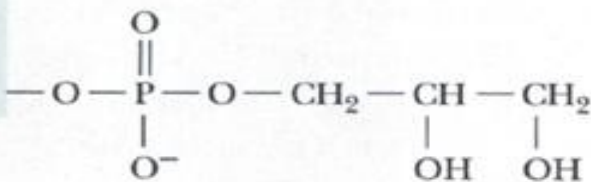
Phosphatidylglycerol
