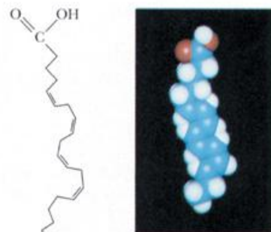
Arachidonic acid
