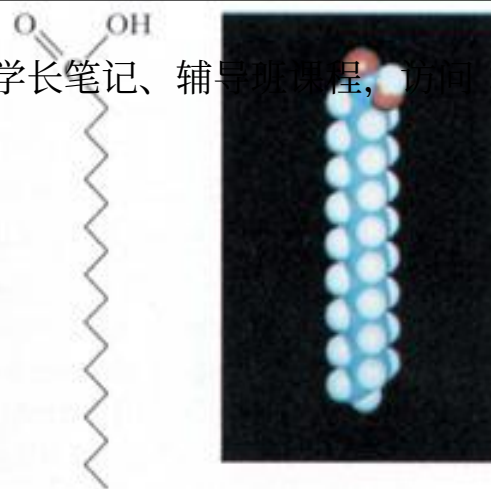
Stearic acid
